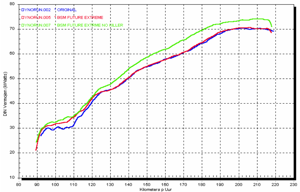
HONDA CB 1000
